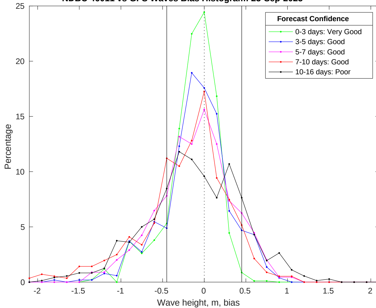
NDBC 46011 vs GFS Waves Bias Histogram: 23-Sep-2025
