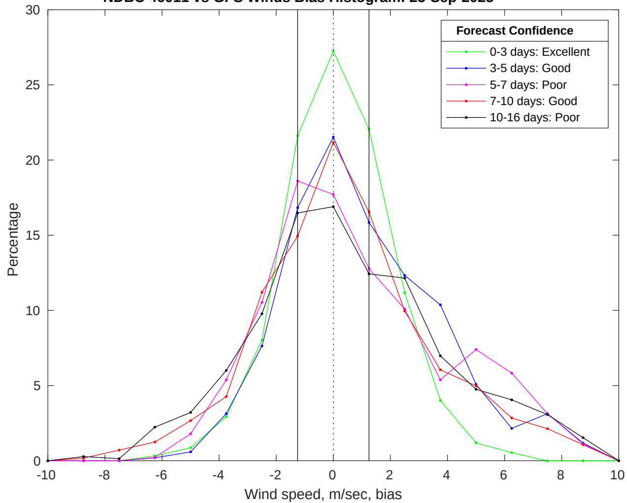
NDBC 46011 vs GFS Winds Bias Histogram: 23-Sep-2025
