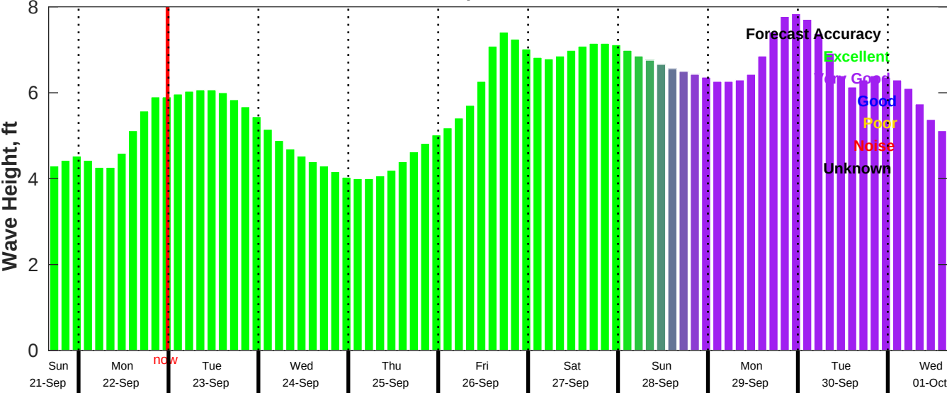
CMEMS Wave Forecast for NDBC 46011 from 21-Sep-2025 16:00:00 to 01-Oct-2025 16:00:00
