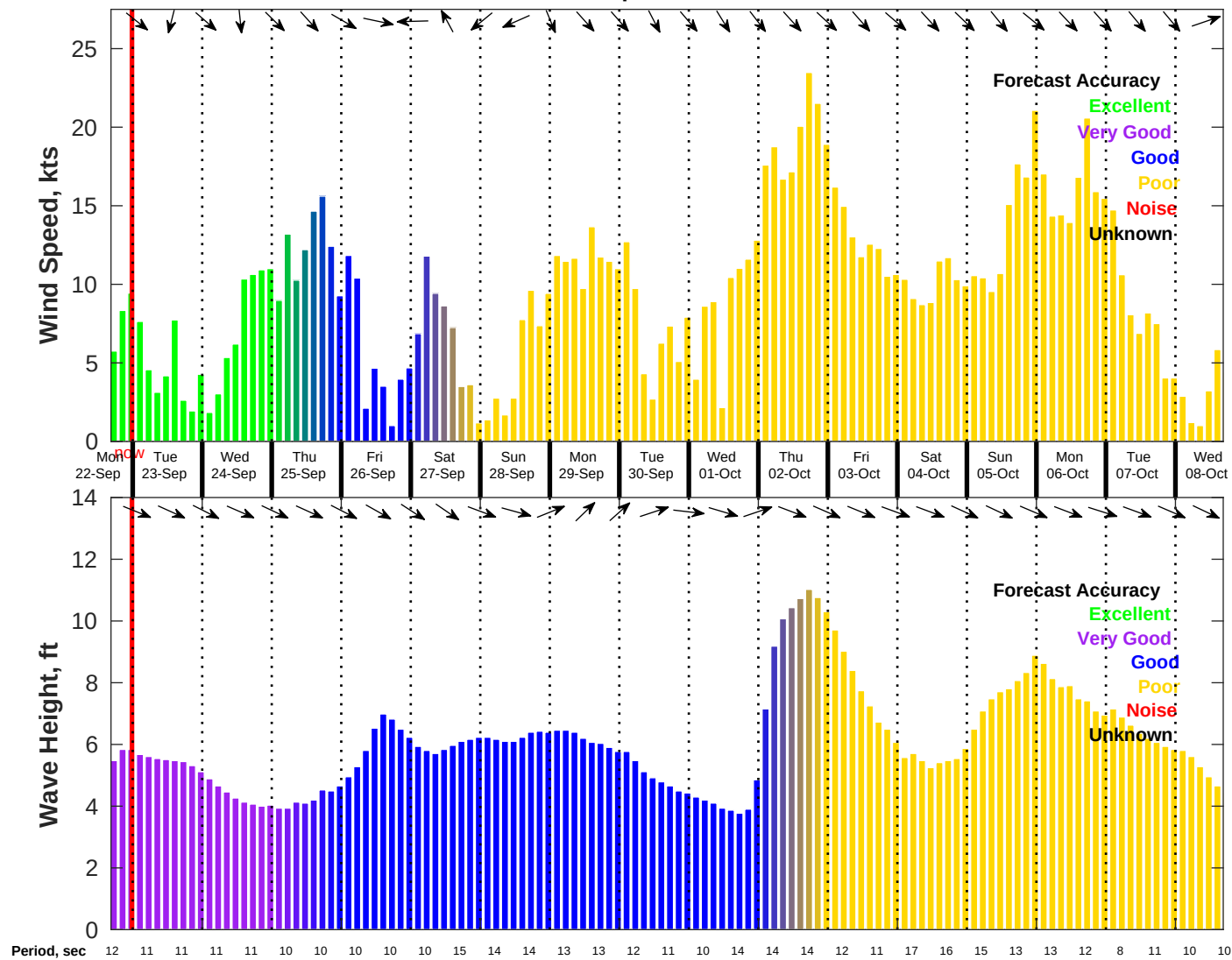
Wind & Wave Forecast for NDBC 46011 from 22-Sep-2025 16:00:00 to 08-Oct-2025 16:00:00
