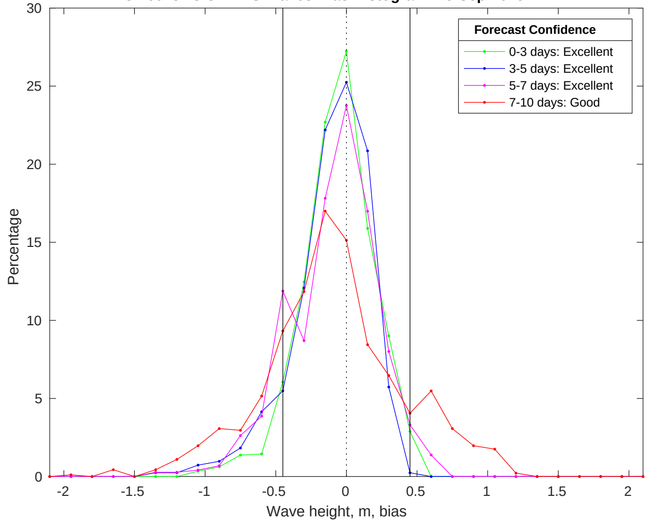
NDBC 46028 vs CMEMS Waves Bias Histogram: 23-Sep-2025
