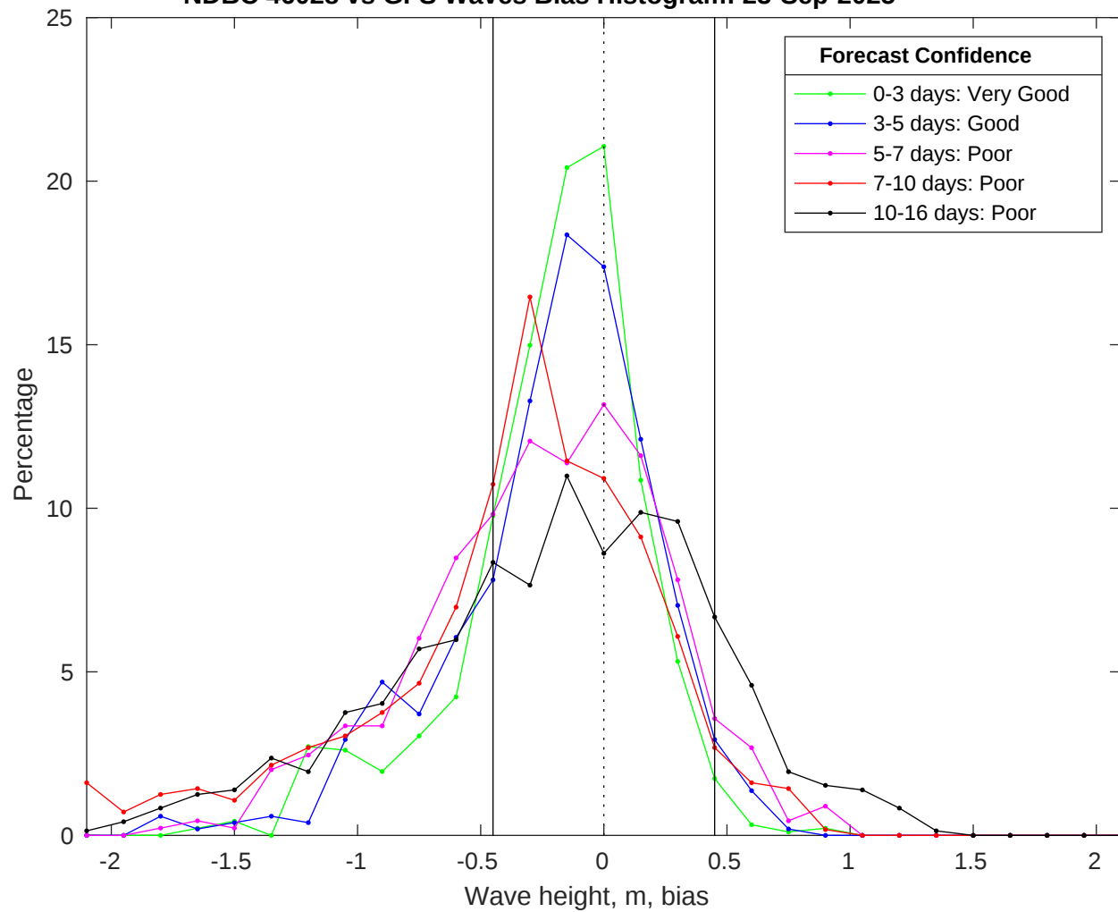
NDBC 46028 vs GFS Waves Bias Histogram: 23-Sep-2025
