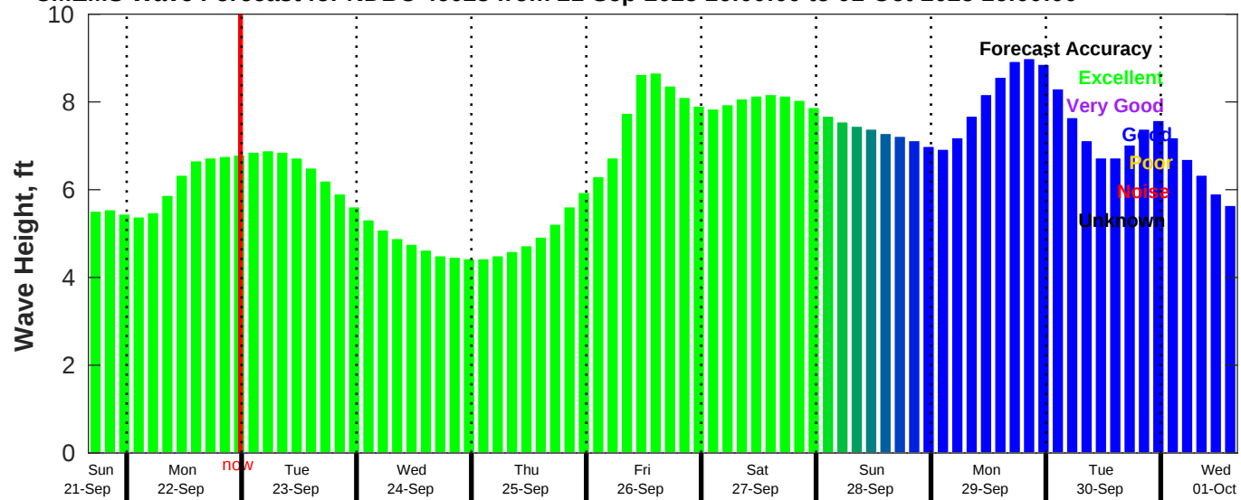
CMEMS Wave Forecast for NDBC 46028 from 21-Sep-2025 16:00:00 to 01-Oct-2025 16:00:00
