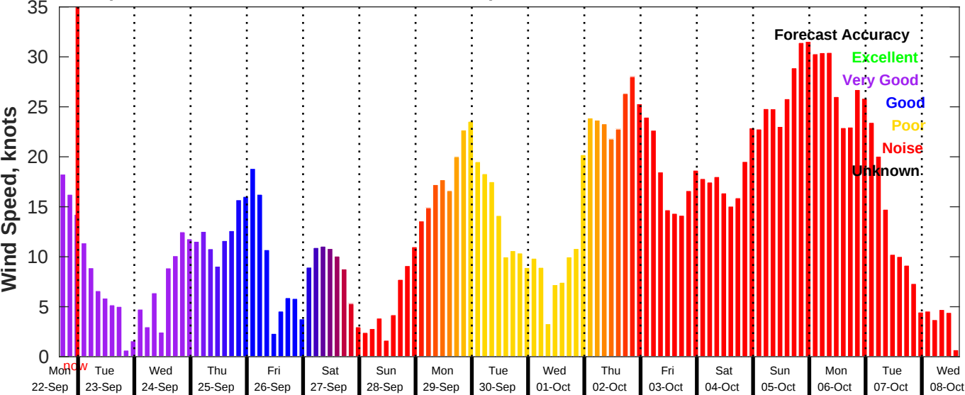
GFS Wind Speed Forecast for NDBC 46028 from 22-Sep-2025 16:00:00 to 08-Oct-2025 16:00:00
