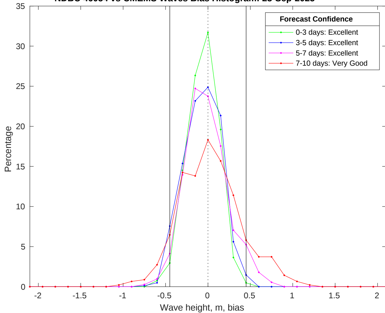
NDBC 46054 vs CMEMS Waves Bias Histogram: 23-Sep-2025
