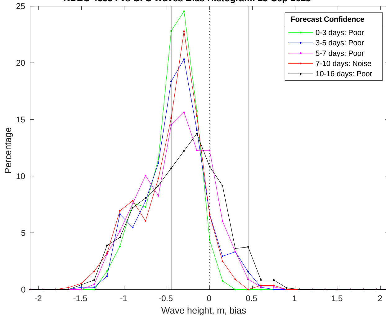
NDBC 46054 vs GFS Waves Bias Histogram: 23-Sep-2025
