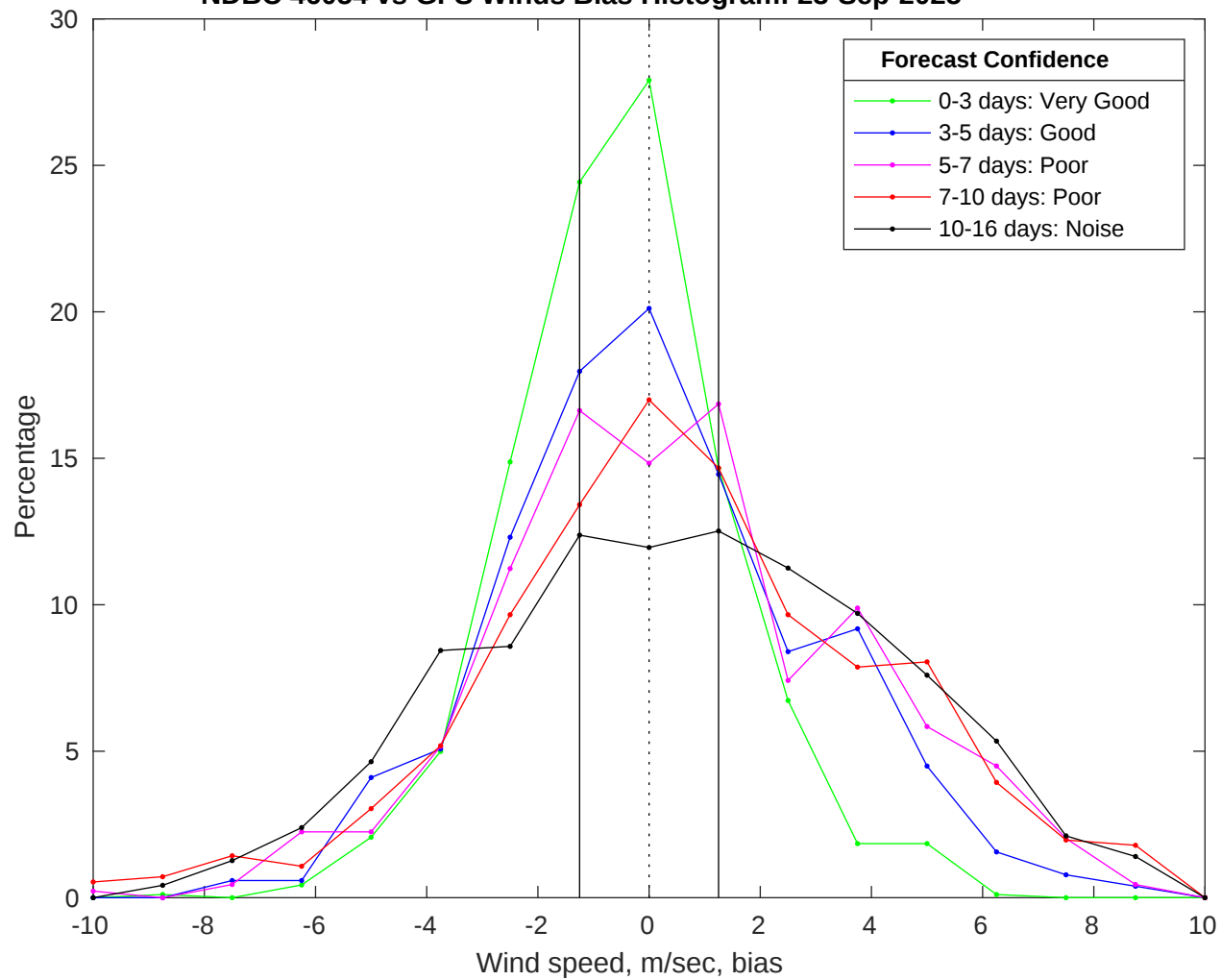
NDBC 46054 vs GFS Winds Bias Histogram: 23-Sep-2025
