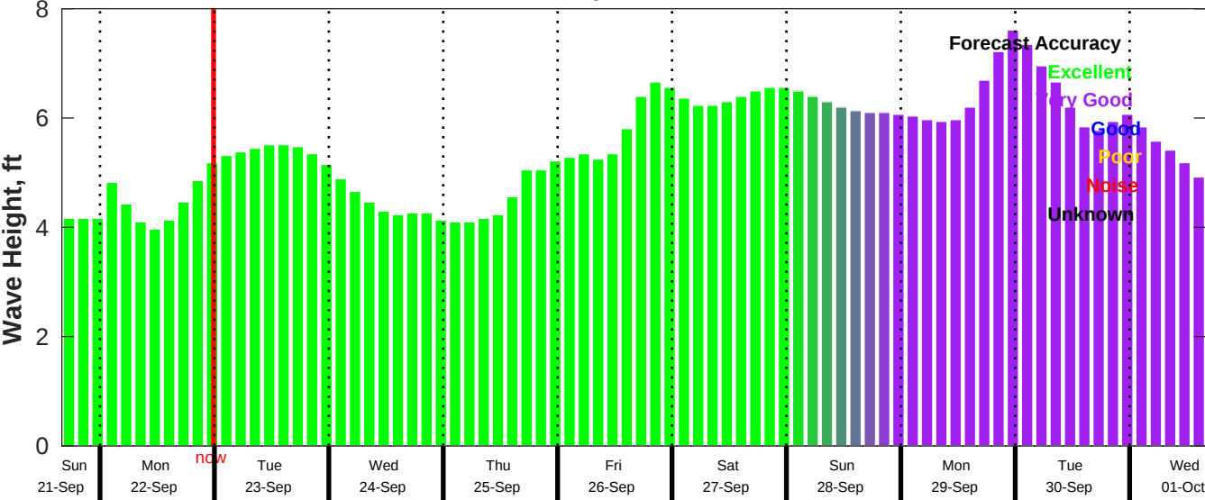
CMEMS Wave Forecast for NDBC 46054 from 21-Sep-2025 16:00:00 to 01-Oct-2025 16:00:00
