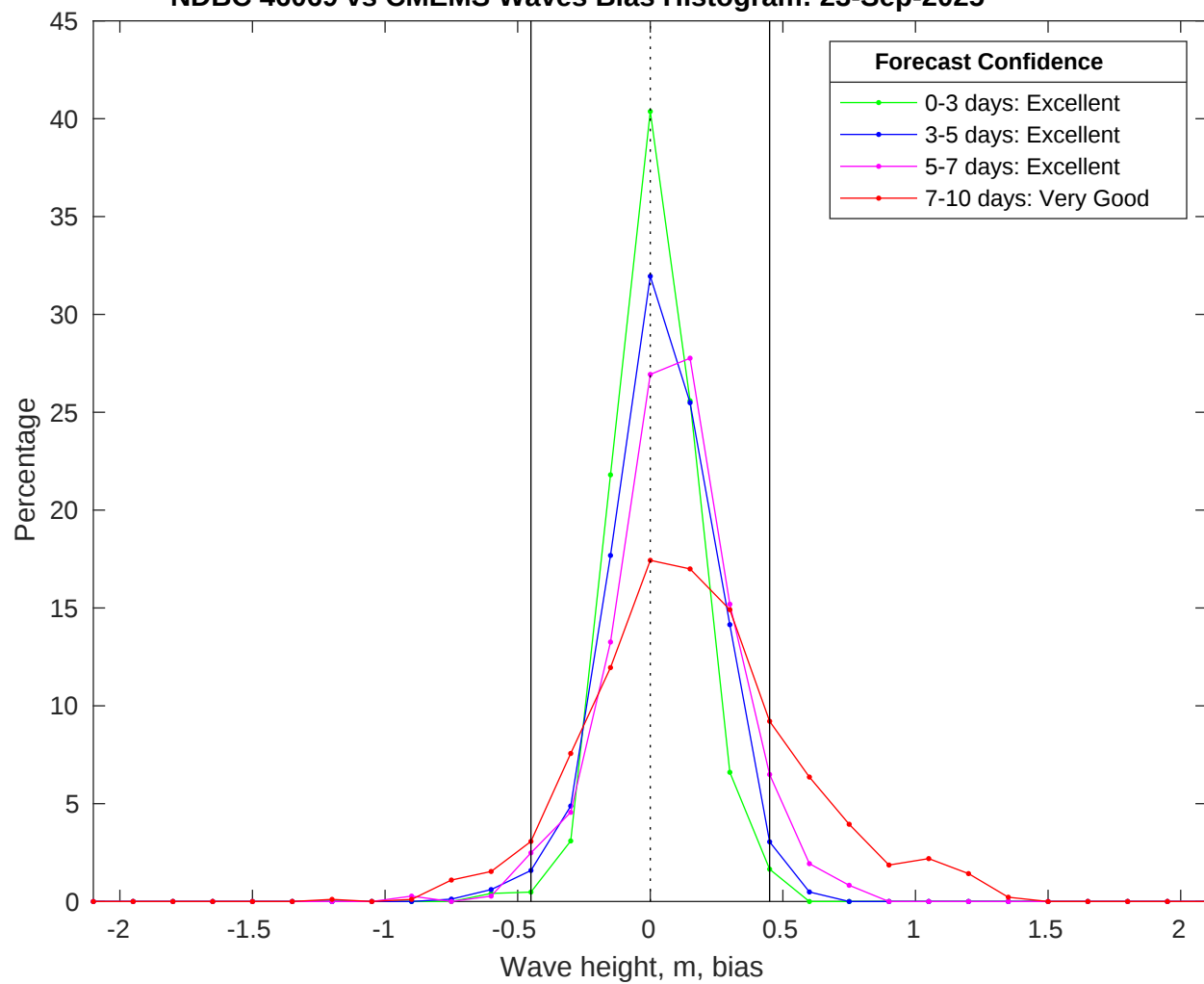
NDBC 46069 vs CMEMS Waves Bias Histogram: 23-Sep-2025
