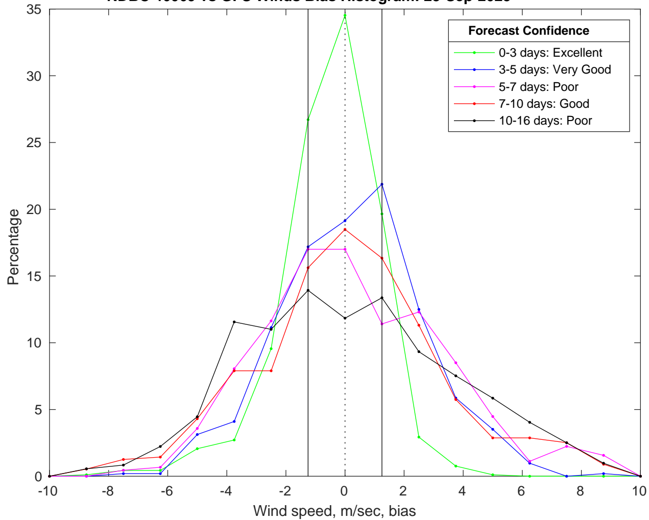
NDBC 46069 vs GFS Winds Bias Histogram: 23-Sep-2025
