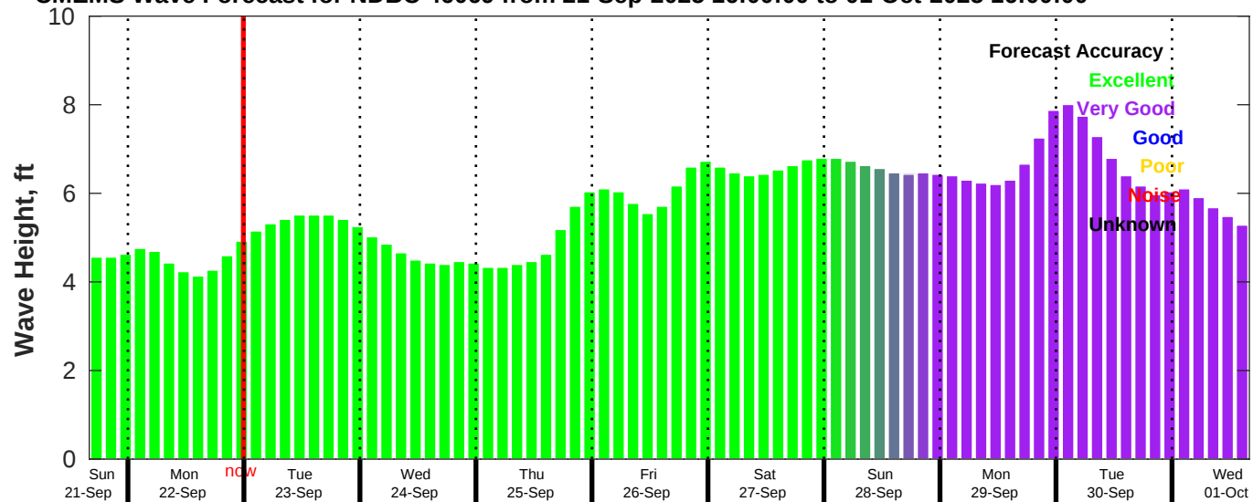
CMEMS Wave Forecast for NDBC 46069 from 21-Sep-2025 16:00:00 to 01-Oct-2025 16:00:00
