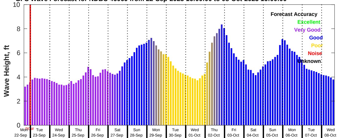
GFS Wave Forecast for NDBC 46069 from 22-Sep-2025 16:00:00 to 08-Oct-2025 16:00:00
