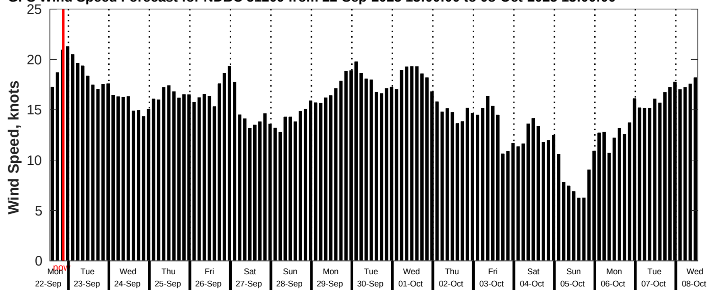
GFS Wind Speed Forecast for NDBC 51209 from 22-Sep-2025 13:00:00 to 08-Oct-2025 13:00:00
