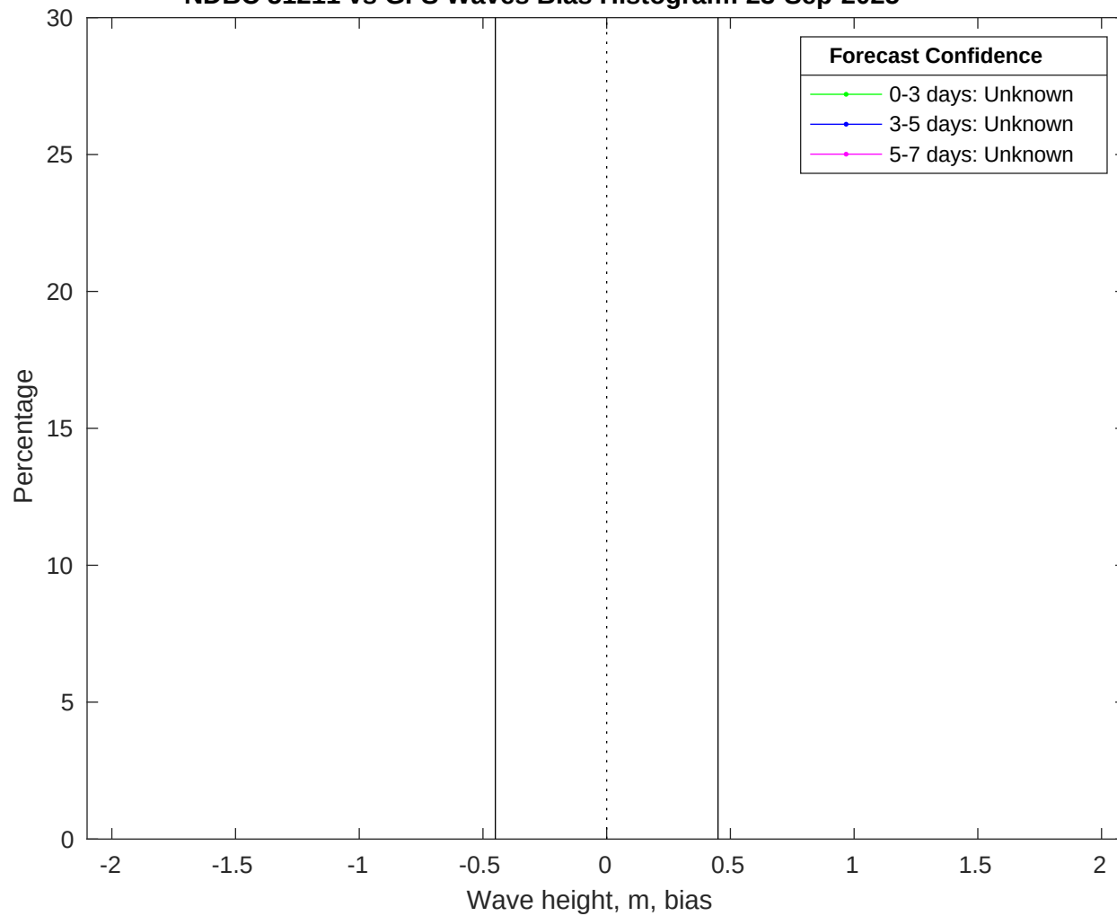
NDBC 51211 vs GFS Waves Bias Histogram: 23-Sep-2025
