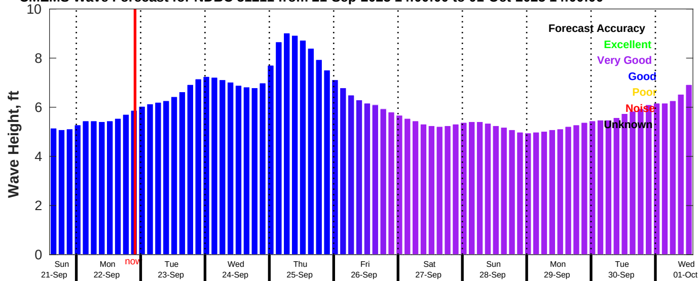
CMEMS Wave Forecast for NDBC 51211 from 21-Sep-2025 14:00:00 to 01-Oct-2025 14:00:00
