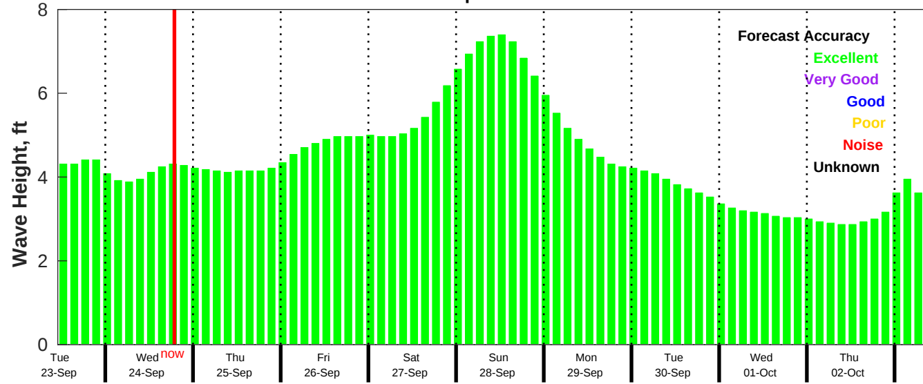
CMEMS Wave Forecast for NDBC 52211 from 22-Sep-2025 11:00:00 to 02-Oct-2025 11:00:00
