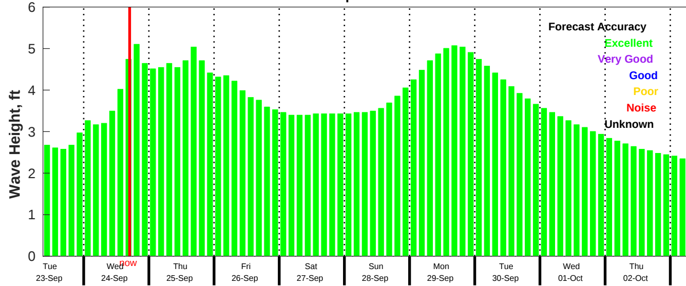
CMEMS Wave Forecast for NDBC 52212 from 22-Sep-2025 09:00:00 to 02-Oct-2025 09:00:00
