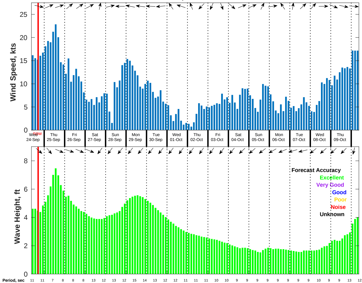
Wind & Wave Forecast for NDBC 52212 from 23-Sep-2025 09:00:00 to 09-Oct-2025 09:00:00
