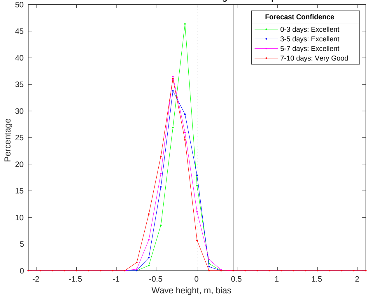
NDBC 52213 vs CMEMS Waves Bias Histogram: 23-Sep-2025
