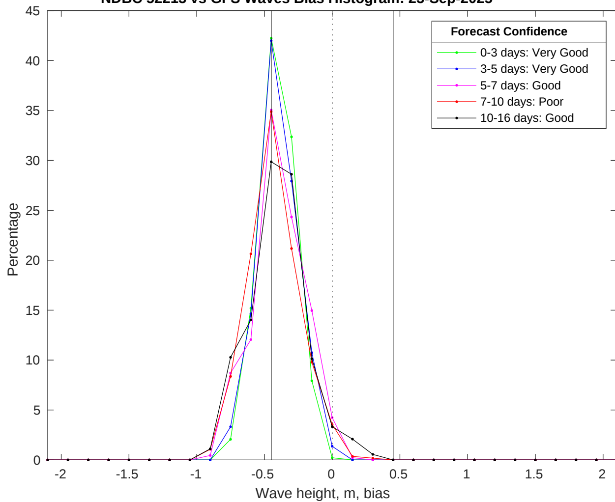
NDBC 52213 vs GFS Waves Bias Histogram: 23-Sep-2025
