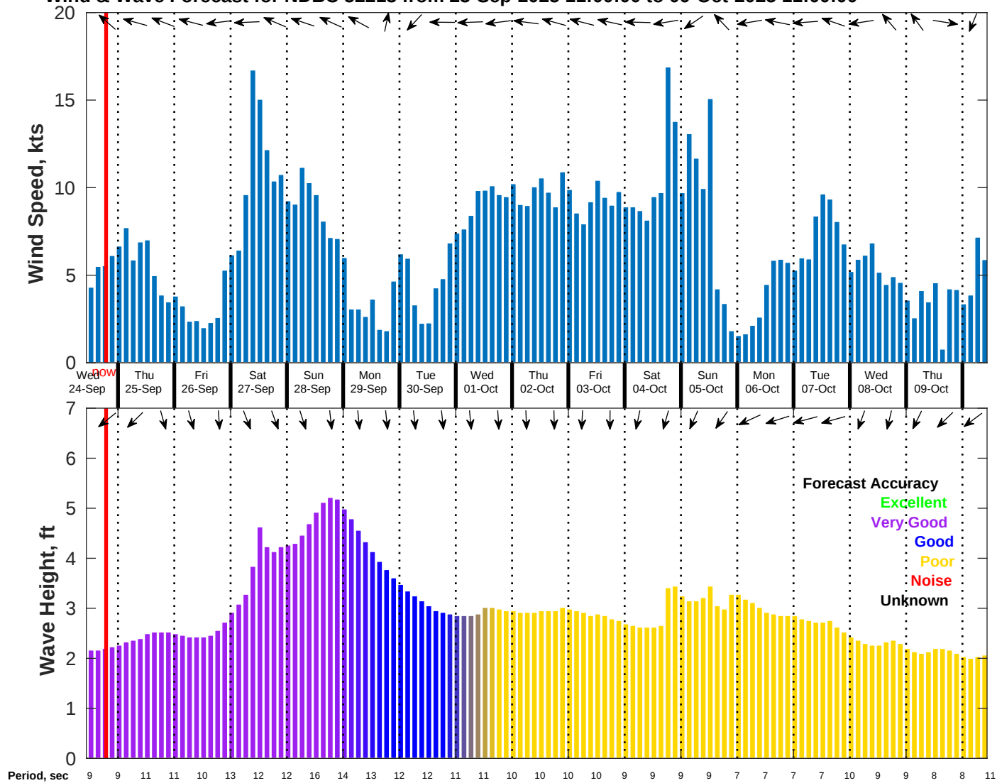
Wind & Wave Forecast for NDBC 52213 from 23-Sep-2025 11:00:00 to 09-Oct-2025 11:00:00
