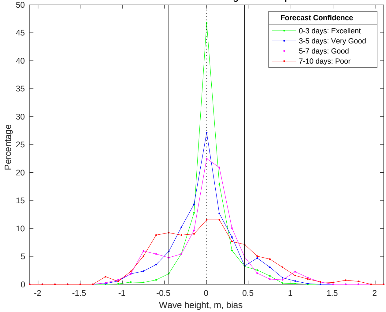
NDBC 41004 vs CMEMS Waves Bias Histogram: 24-Sep-2025
