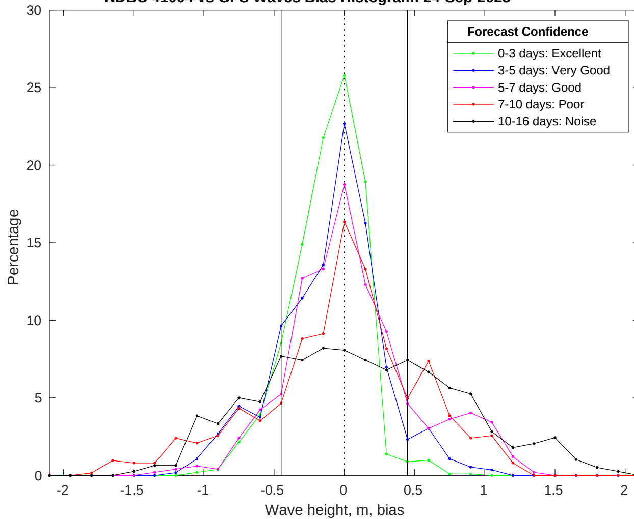
NDBC 41004 vs GFS Waves Bias Histogram: 24-Sep-2025
