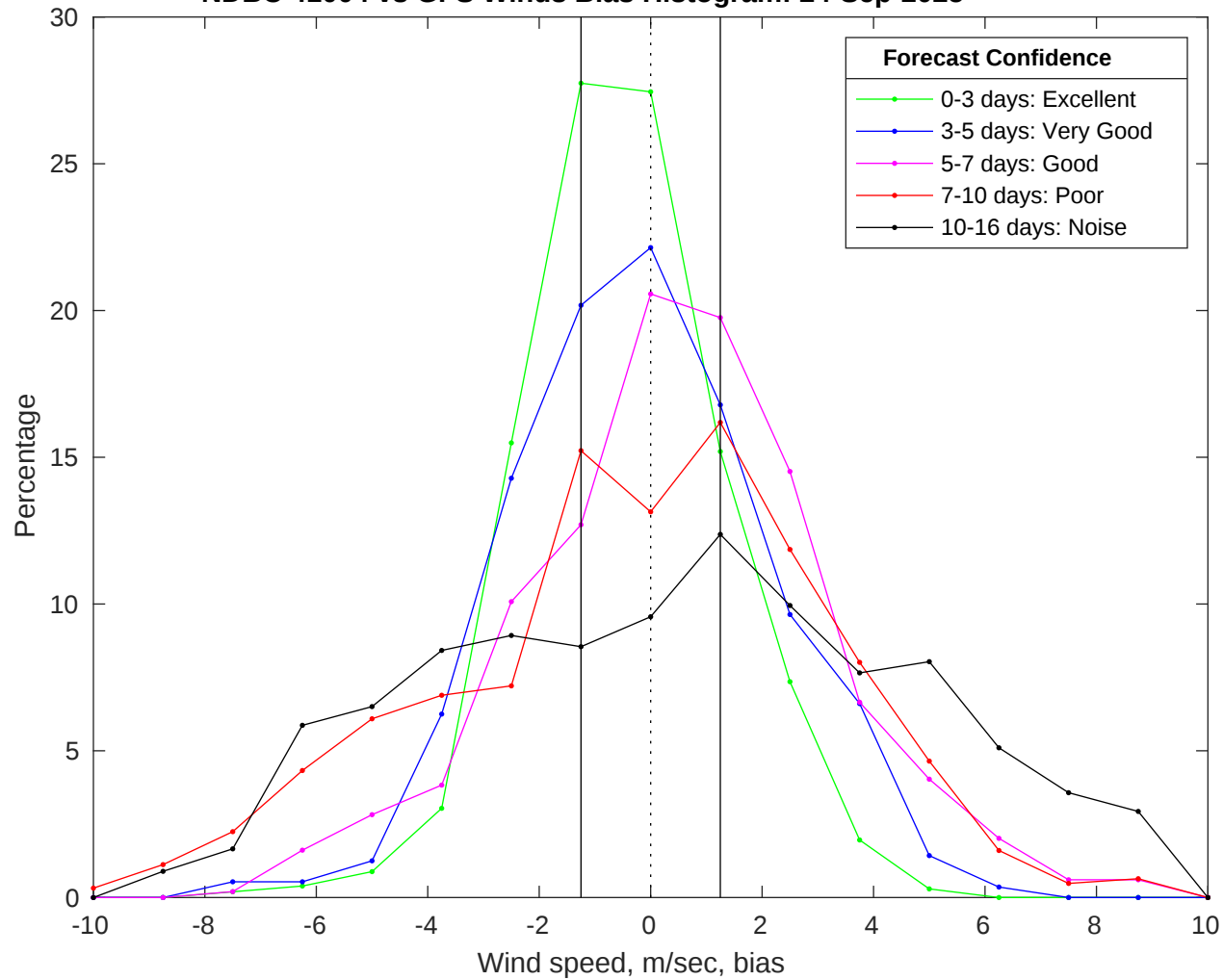
NDBC 41004 vs GFS Winds Bias Histogram: 24-Sep-2025
