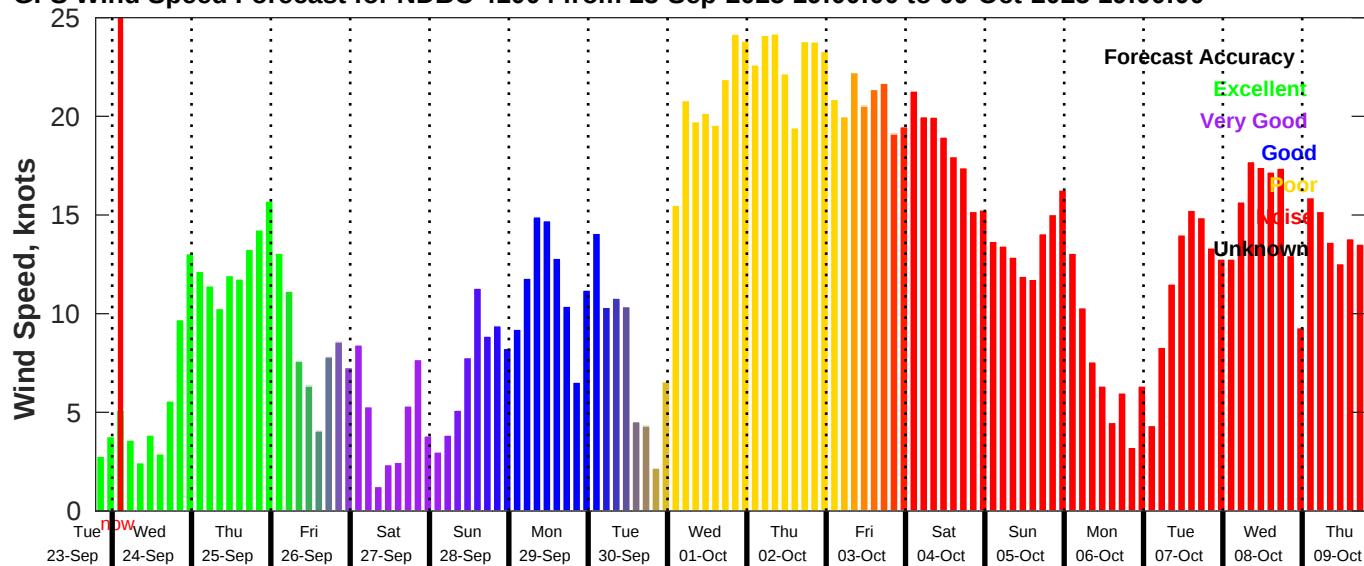
GFS Wind Speed Forecast for NDBC 41004 from 23-Sep-2025 19:00:00 to 09-Oct-2025 19:00:00
