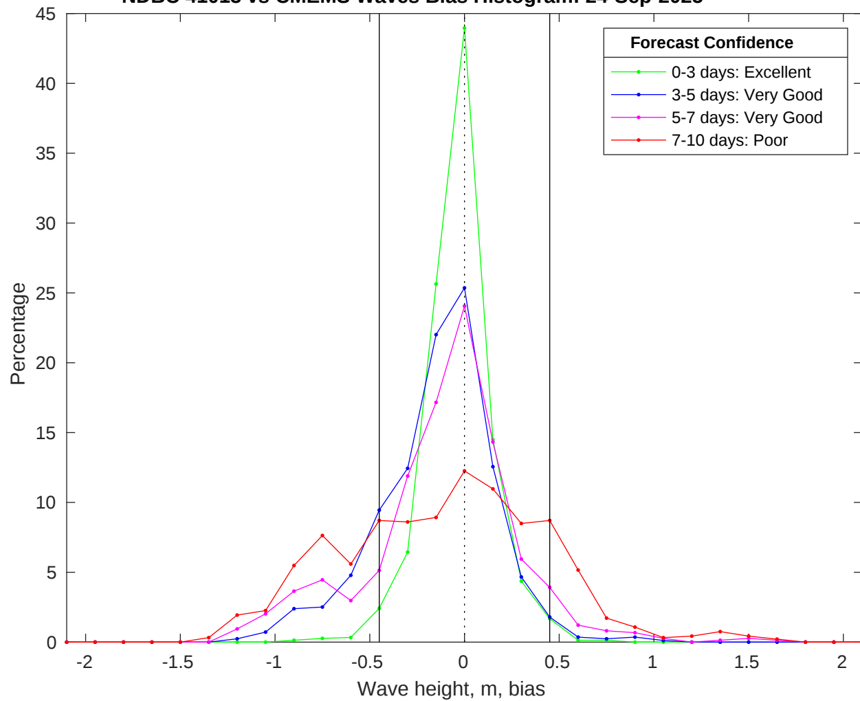
NDBC 41013 vs CMEMS Waves Bias Histogram: 24-Sep-2025
