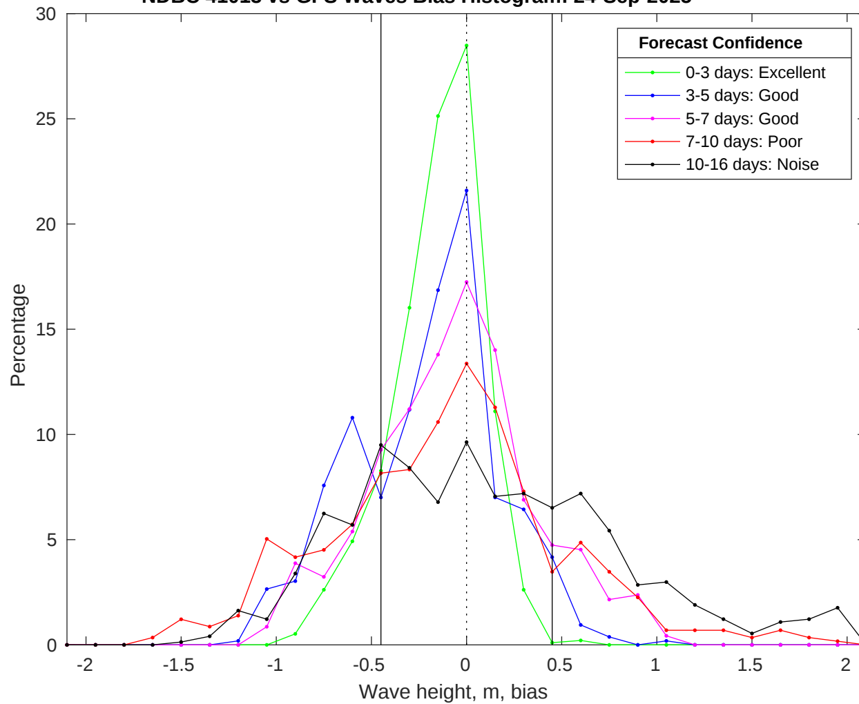
NDBC 41013 vs GFS Waves Bias Histogram: 24-Sep-2025
