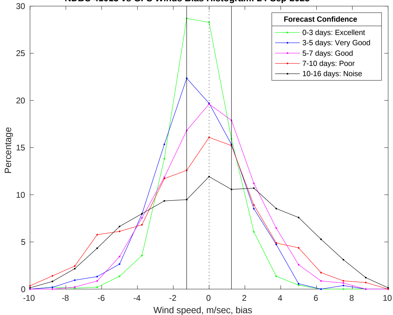
NDBC 41013 vs GFS Winds Bias Histogram: 24-Sep-2025
