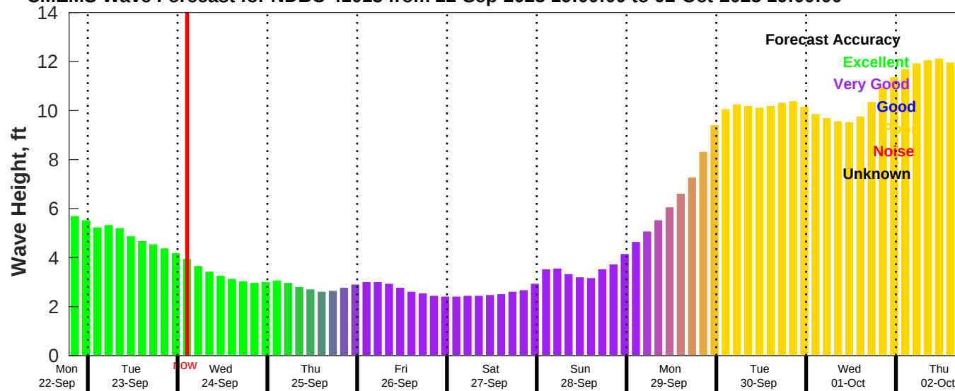
CMEMS Wave Forecast for NDBC 41013 from 22-Sep-2025 19:00:00 to 02-Oct-2025 19:00:00
