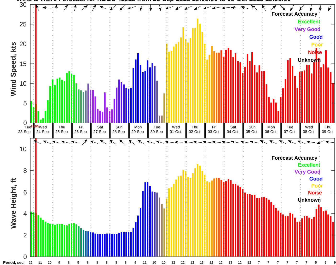
Wind & Wave Forecast for NDBC 41013 from 23-Sep-2025 19:00:00 to 09-Oct-2025 19:00:00
