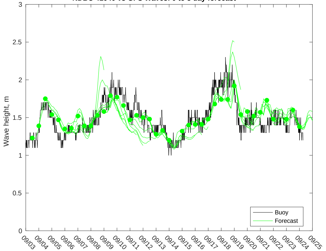
NDBC 41040 vs GFS Waves: 0 to 3 day forecast
