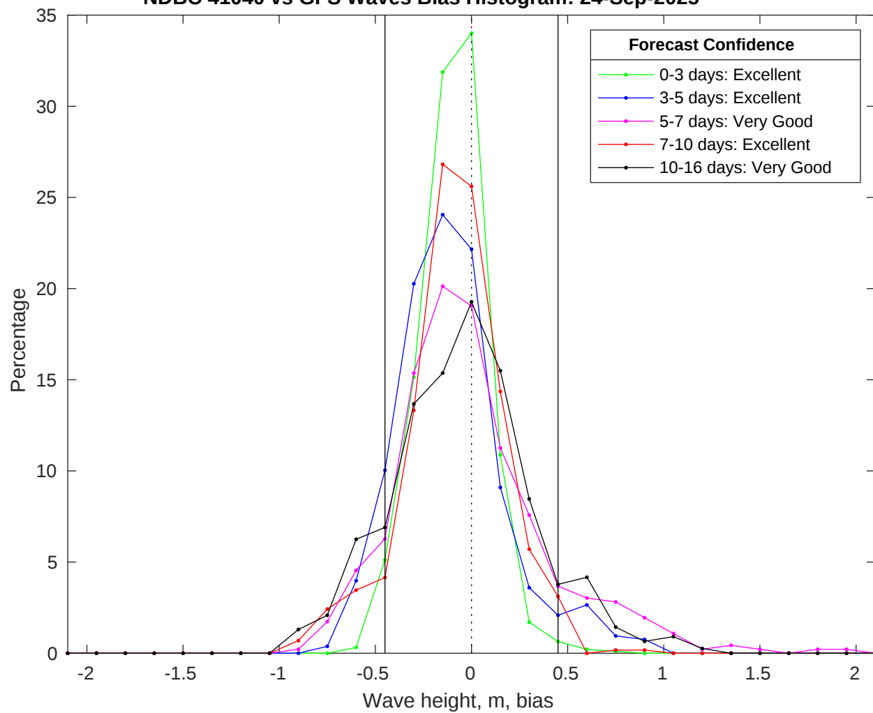
NDBC 41040 vs GFS Waves Bias Histogram: 24-Sep-2025
