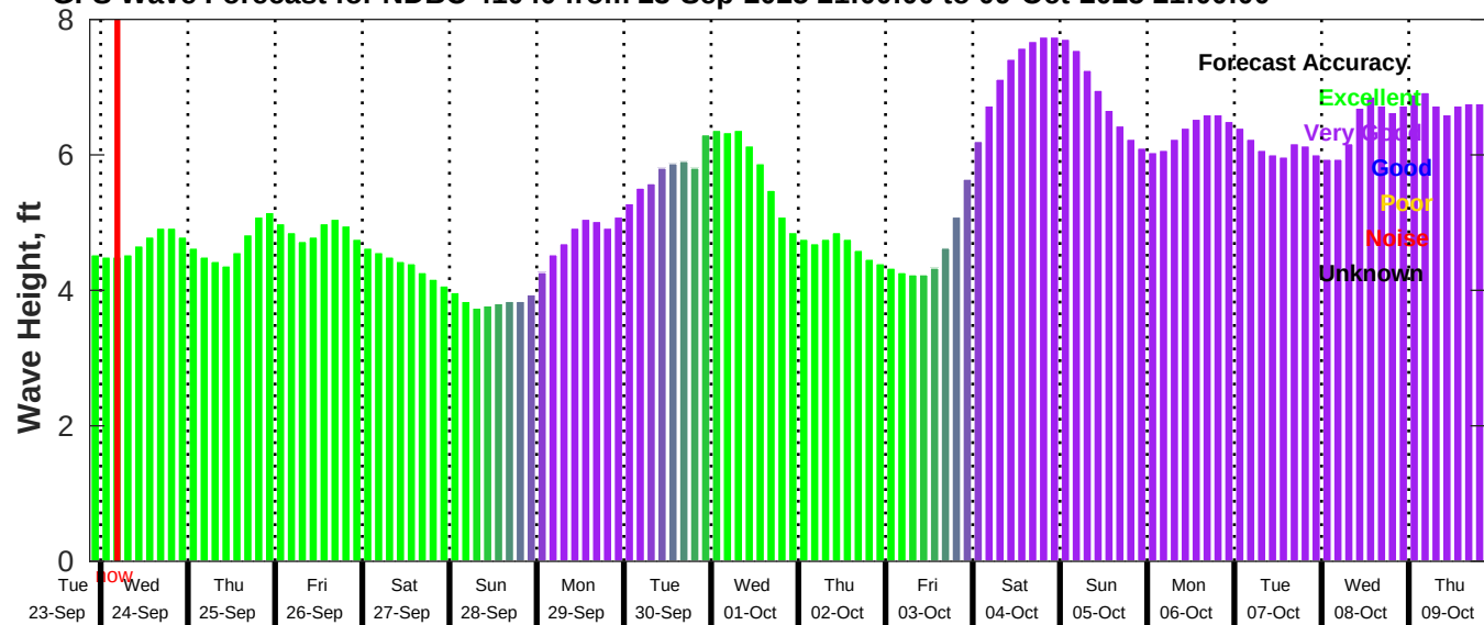
GFS Wave Forecast for NDBC 41040 from 23-Sep-2025 21:00:00 to 09-Oct-2025 21:00:00
