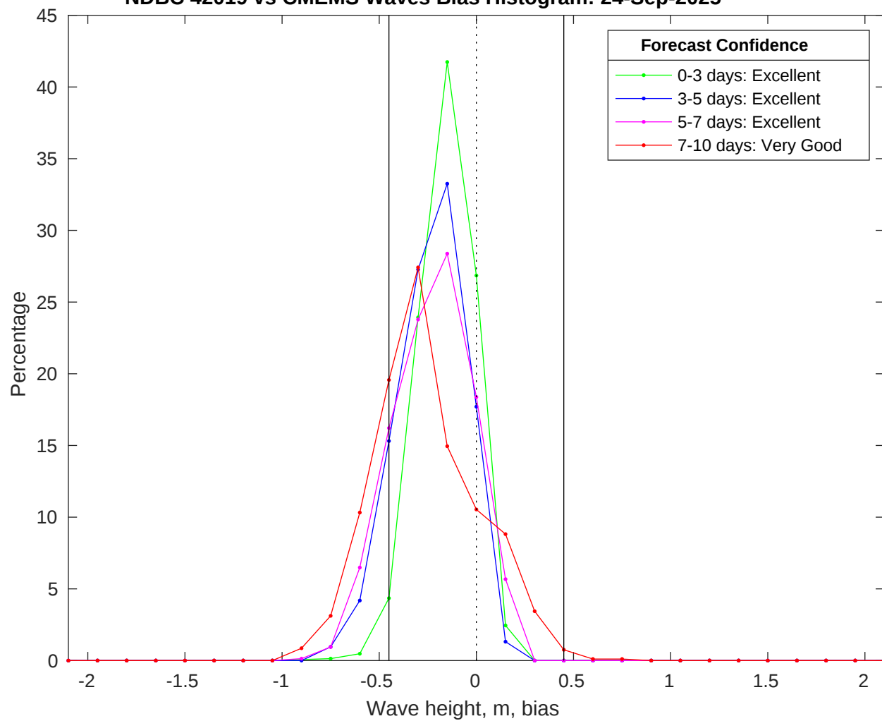
NDBC 42019 vs CMEMS Waves Bias Histogram: 24-Sep-2025
