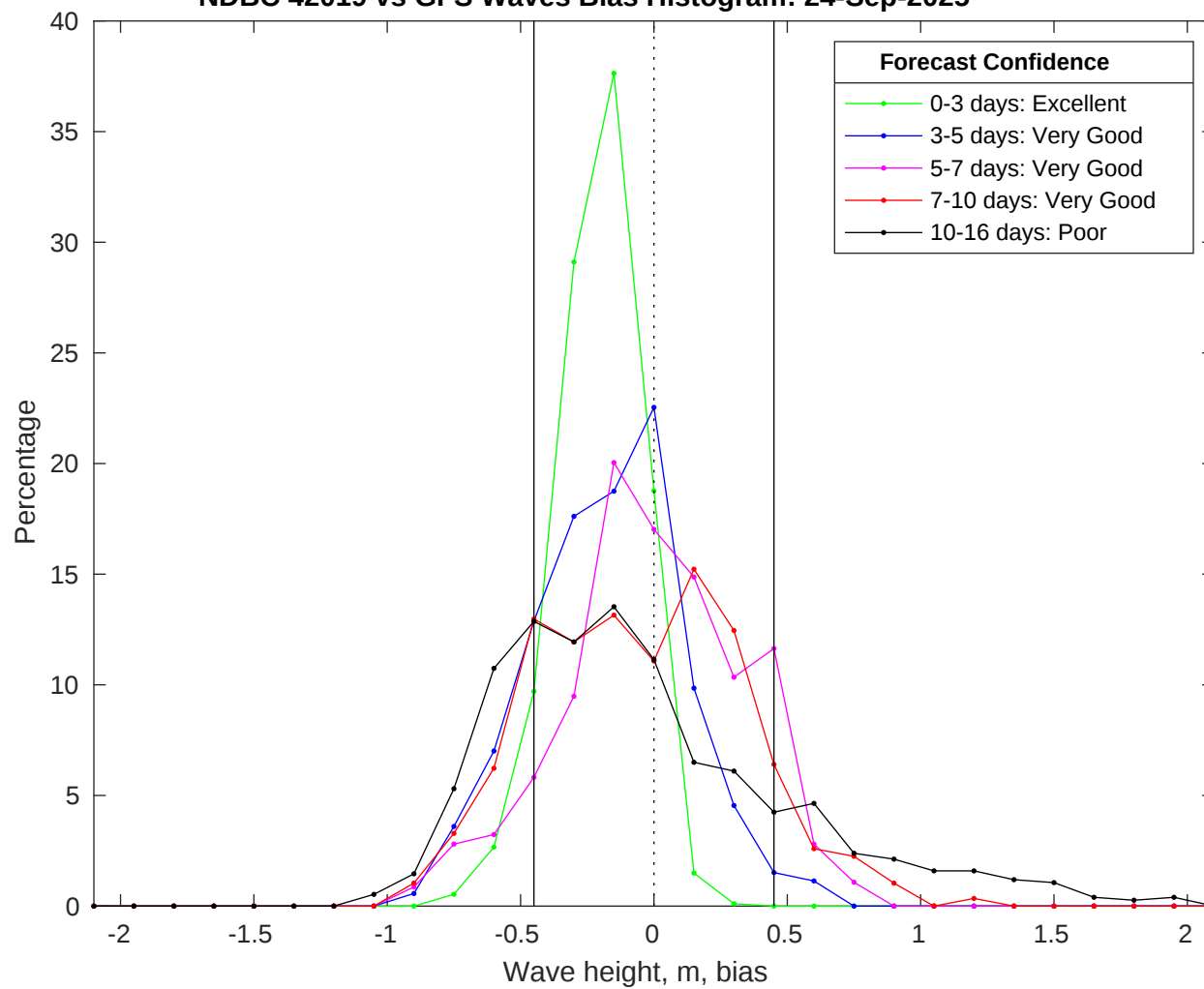
NDBC 42019 vs GFS Waves Bias Histogram: 24-Sep-2025
