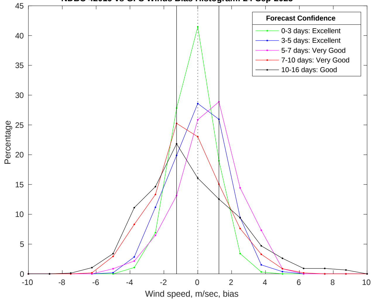
NDBC 42019 vs GFS Winds Bias Histogram: 24-Sep-2025
