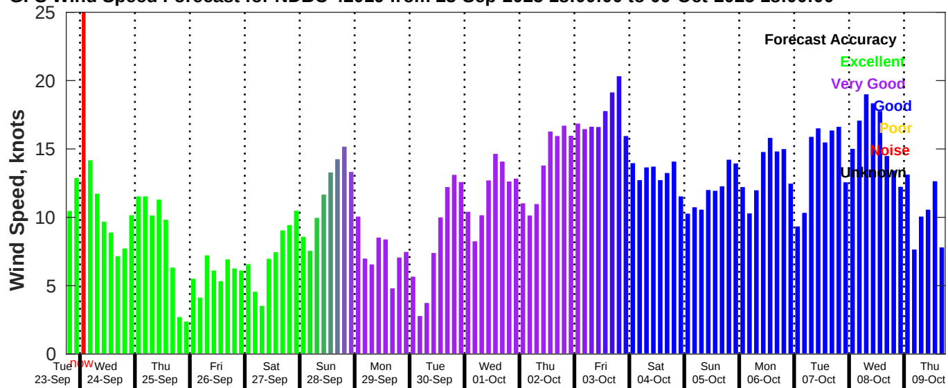
GFS Wind Speed Forecast for NDBC 42019 from 23-Sep-2025 18:00:00 to 09-Oct-2025 18:00:00
