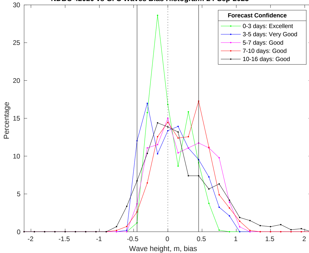
NDBC 42020 vs GFS Waves Bias Histogram: 24-Sep-2025
