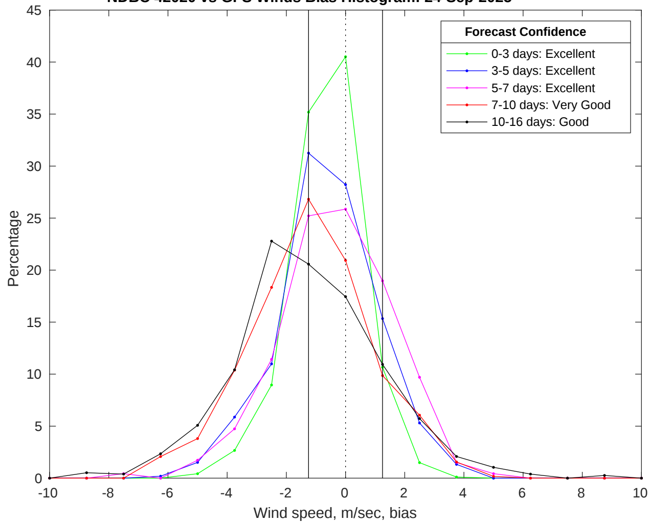
NDBC 42020 vs GFS Winds Bias Histogram: 24-Sep-2025
