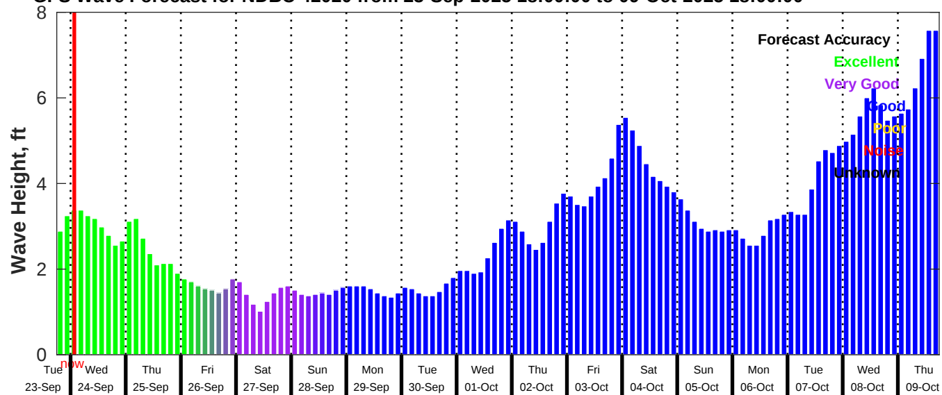
GFS Wave Forecast for NDBC 42020 from 23-Sep-2025 18:00:00 to 09-Oct-2025 18:00:00
