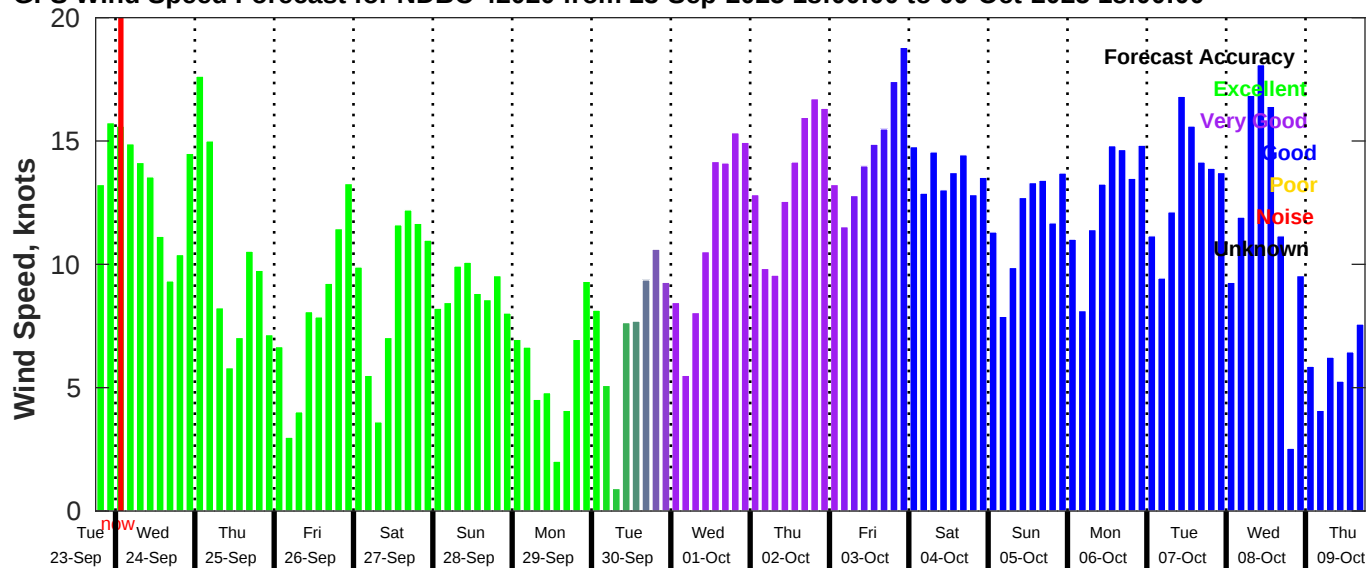
GFS Wind Speed Forecast for NDBC 42020 from 23-Sep-2025 18:00:00 to 09-Oct-2025 18:00:00
