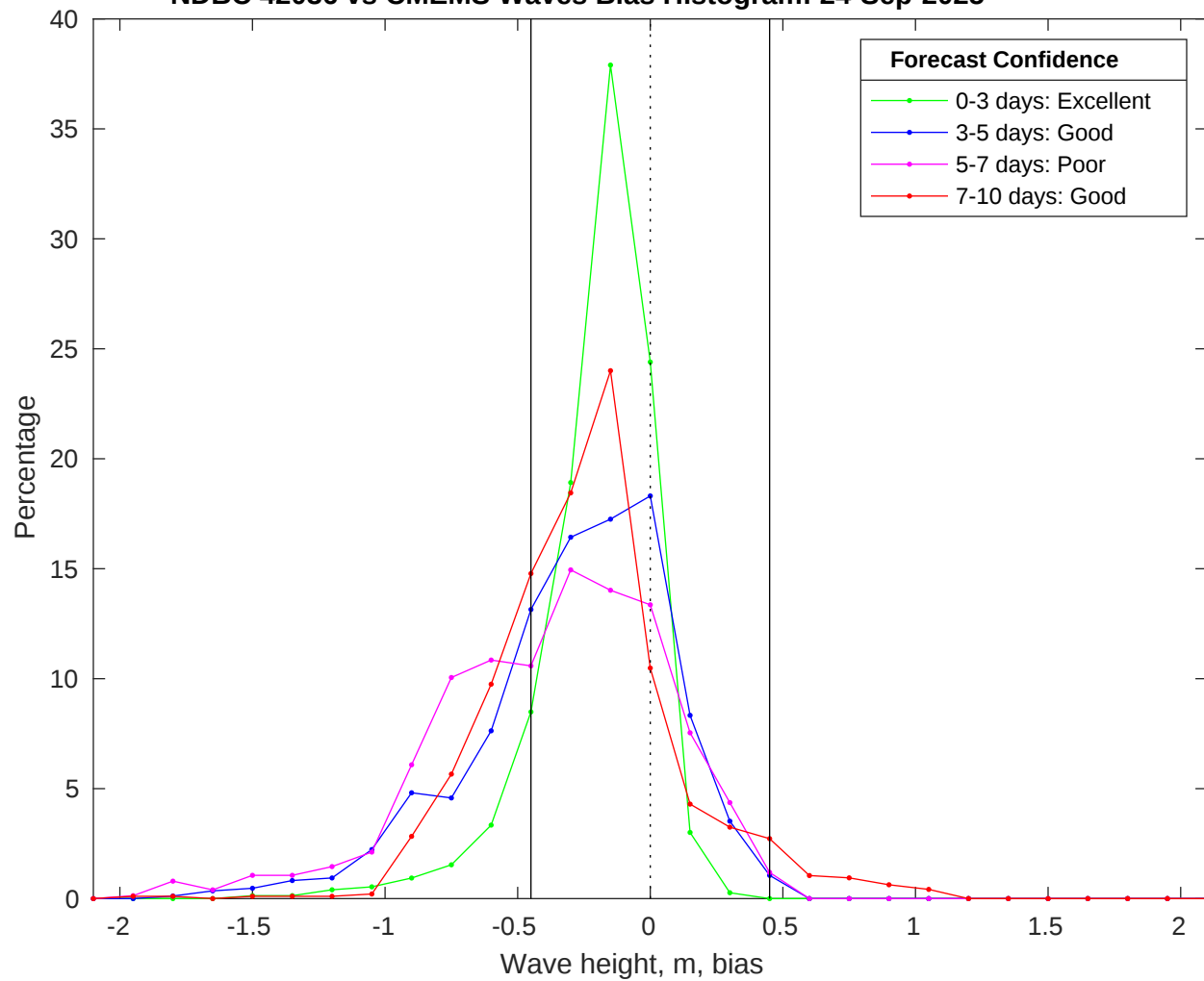
NDBC 42036 vs CMEMS Waves Bias Histogram: 24-Sep-2025
