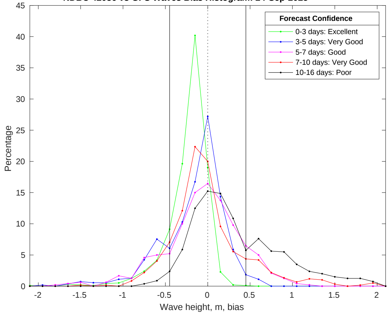
NDBC 42036 vs GFS Waves Bias Histogram: 24-Sep-2025
