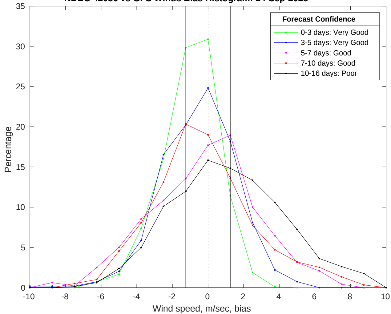
NDBC 42036 vs GFS Winds Bias Histogram: 24-Sep-2025
