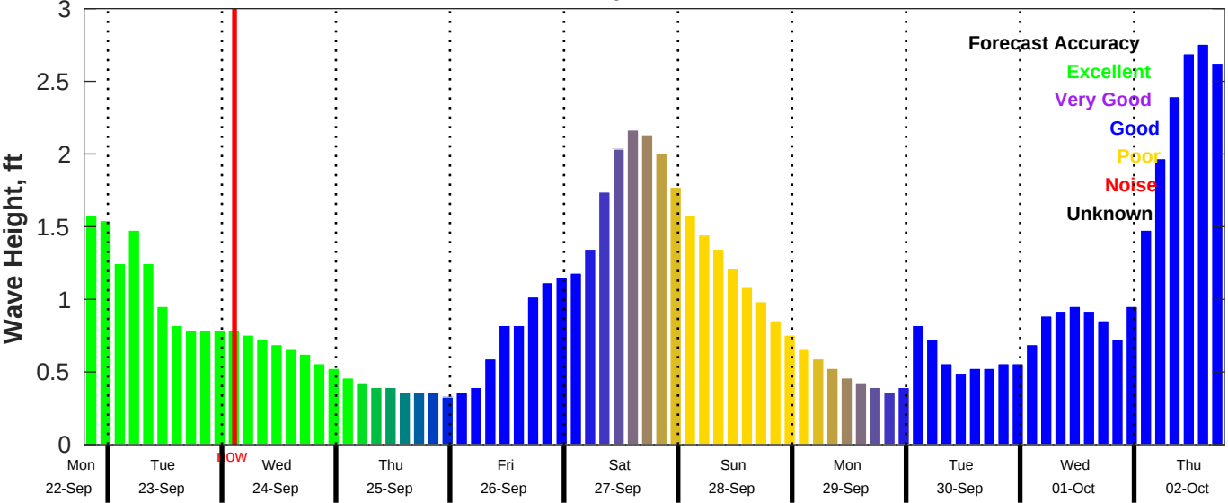
CMEMS Wave Forecast for NDBC 42036 from 22-Sep-2025 19:00:00 to 02-Oct-2025 19:00:00
