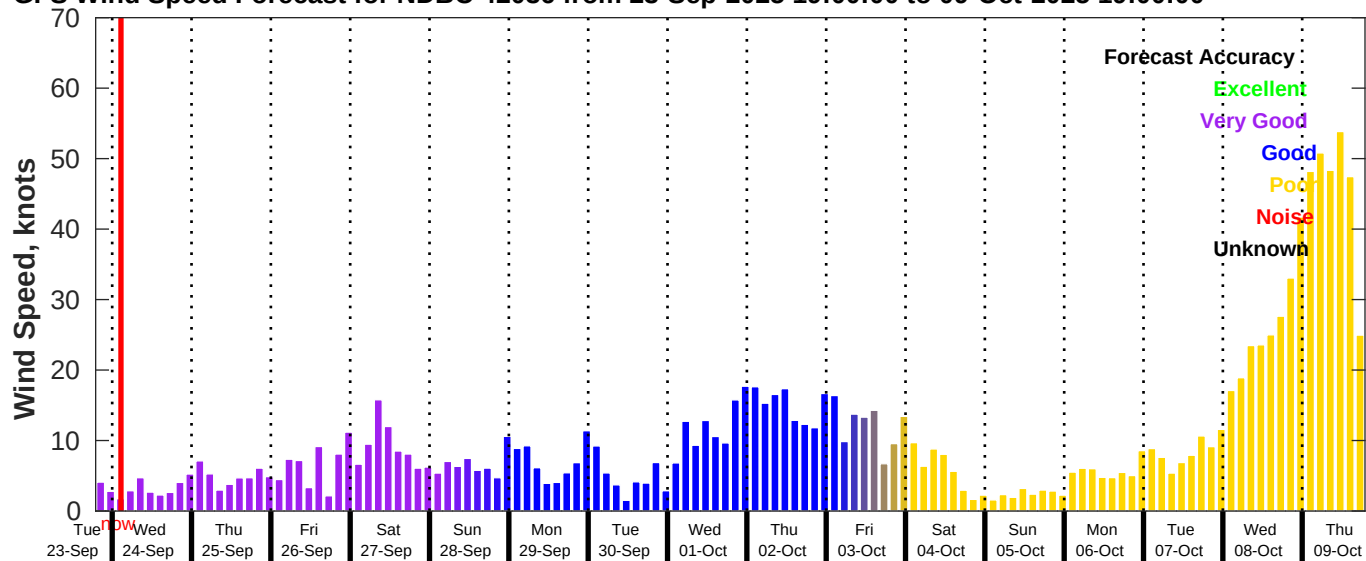
GFS Wind Speed Forecast for NDBC 42036 from 23-Sep-2025 19:00:00 to 09-Oct-2025 19:00:00
